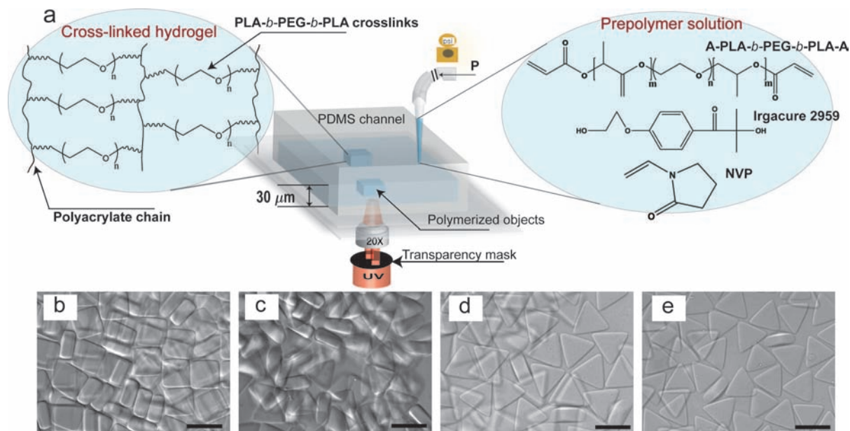
Figure 1. (a) Schematic depicting nonspherical microhydrogel synthesis using stop-flow lithography, chemical structure of the biodegradable diacrylate PLA- b -PEG- b -PLA macromer, photoinitiator, and accelerator (right), and idealized diacrylate PLA- b -PEG- b -PLA hydrogel network after photopolymerization (left). Particles are formed through three steps: (i) a prepolymer solution (diacrylate PLA- b -PEG- b -PLA or PEGDA with Irgacure 2959 and NVP) is flowed through a PDMS channel by a regulated pressure; (ii) the flow is stopped, and particles are polymerized with a desired pulse of UV exposed through a photomask and microscope objective; (iii) the polymerized particles are flushed out of the channel and collected. (b–e) Optical images of the resulting hydrogels: (b) nondegradable hydrogels (rectangles, PEGDA 30 wt %) as the control and (c–e) degradable hydrogels (triangles, diacrylate PLA- b -PEG- b -PLA (c) 30 wt %, (d) 20 wt %, and (e) 10 wt %). Their thicknesses are \sim 26 \mu\text{m} (rectangles, control) and \sim 25 , 22, and 17 \mu\text{m} (triangles, c, d, and e, respectively) Scale bars are all 50 \mu\text{m} . An exposure dose of 0.044 J/cm 2 UV is used for all hydrogel particles shown here.
